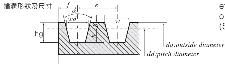
皮帶輪標準(1)V-pulley for Kraft bands with classical V-belts to ISO 5291
